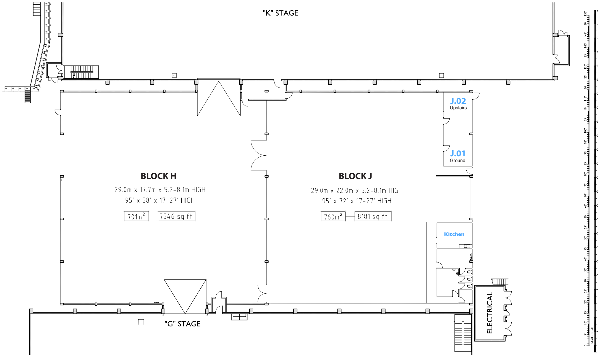
Block H & Block J - Ground Floor Plan SCALE 1:150
