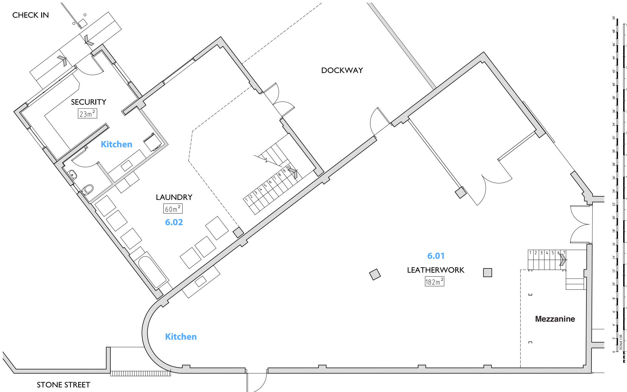
Block Six - Ground Floor Plan SCALE 1:50
